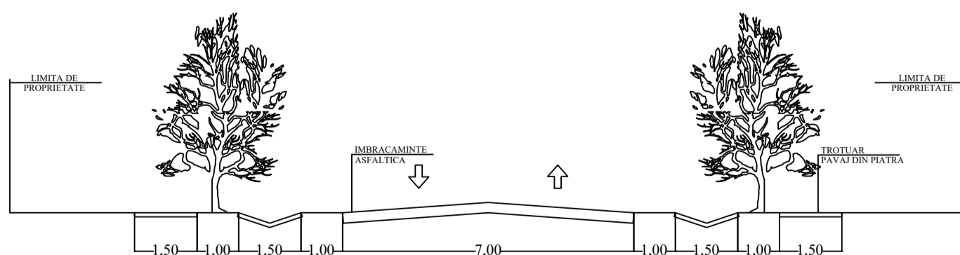
PROFIL TRANSVERSAL DRUM JUDETEAN 1-1
